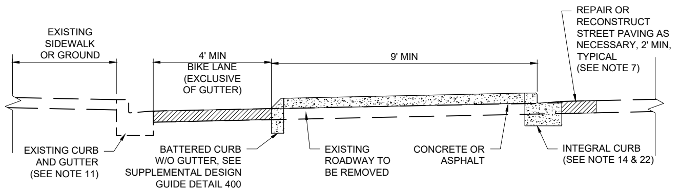
G1 10 TYPICAL SECTION FOR TYPE 2 PROTECTED INTERSECTION WITH EXISTING CURB AND GUTTER
