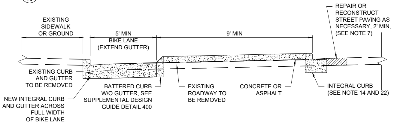
G2 10 TYPICAL SECTION FOR TYPE 2 PROTECTED INTERSECTION WITH REBUILT CURB AND GUTTER
