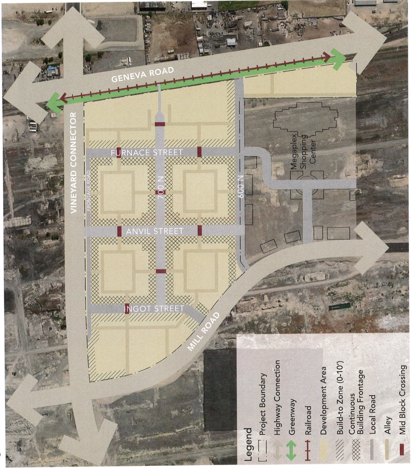
Figure 2.3 - Building Frontage and Build-to Zone
