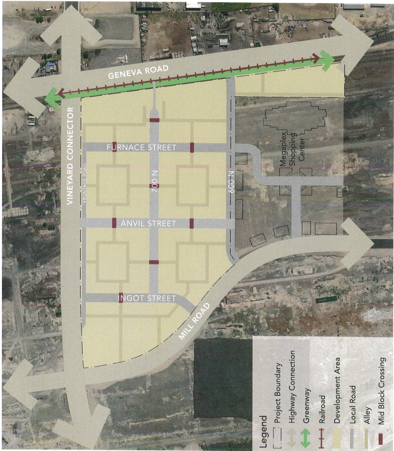
Figure 2.2 - Pedestrian Circulation
