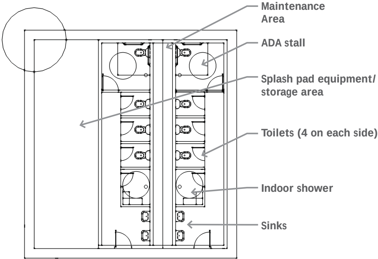
Restroom Floor Plan Concept
