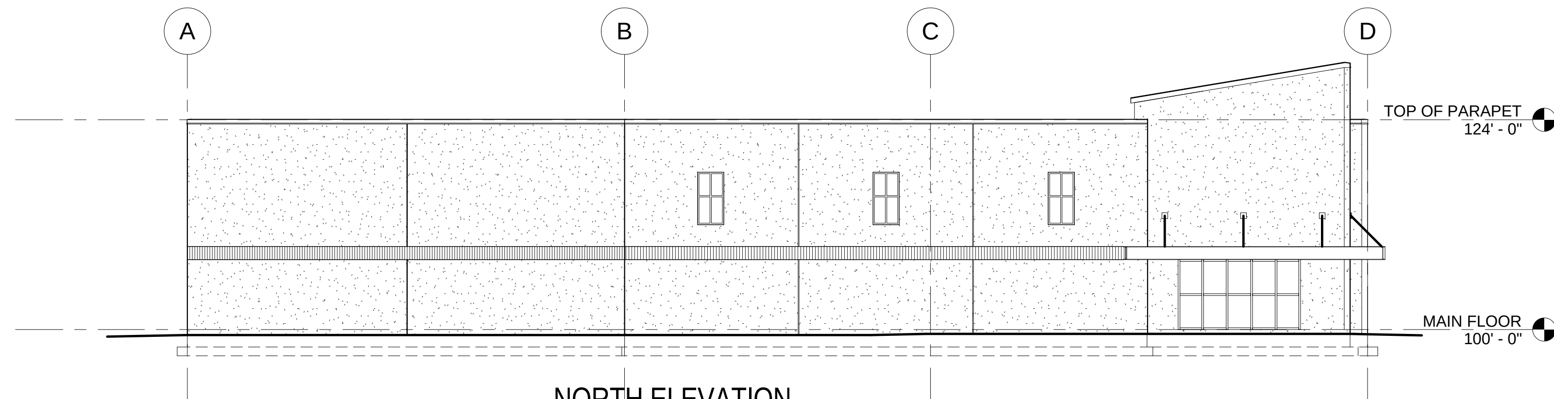
NORTH ELEVATION
