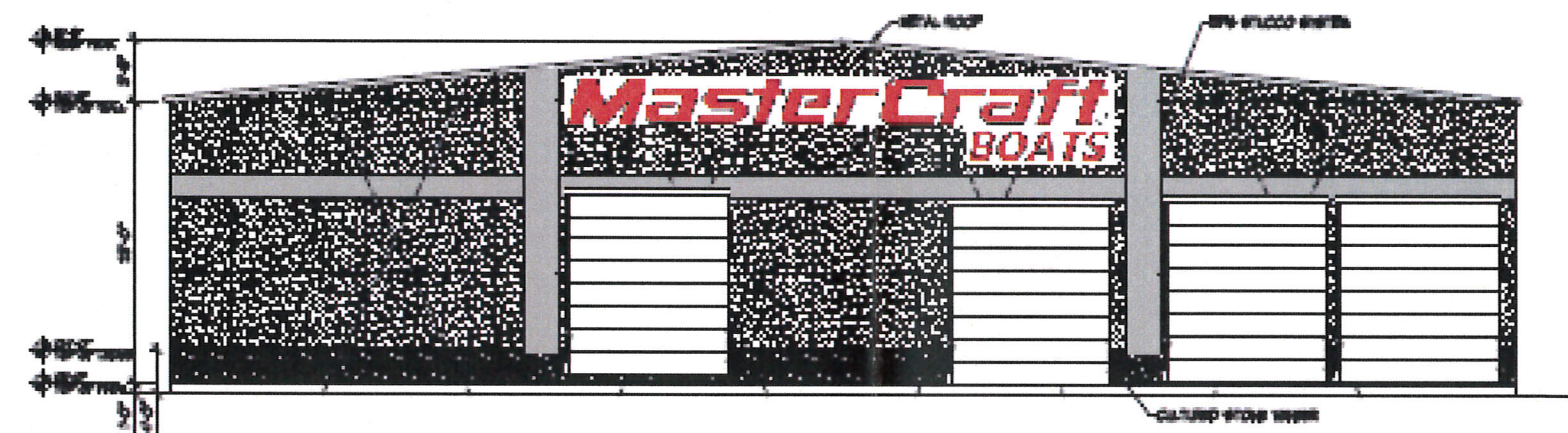
4 New Solid Panel Overhead Doors SIDE ELEVATION 10'-10" 3
