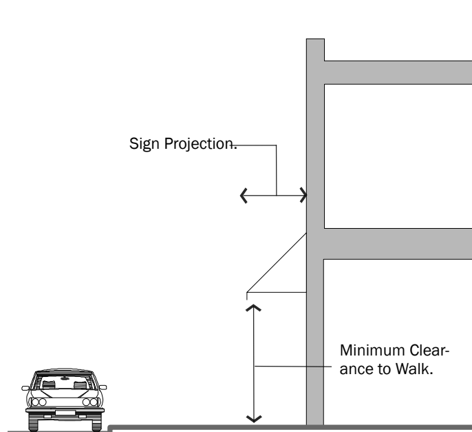
Figure 9.5 (1). Awning Sign.
