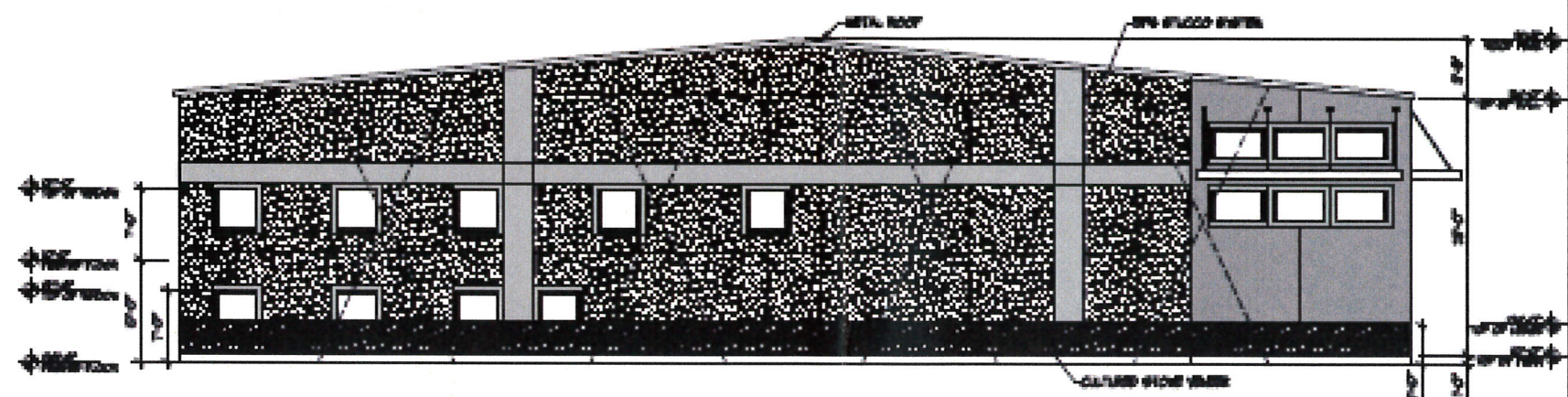
SIDE ELEVATION 10'-10" 4
