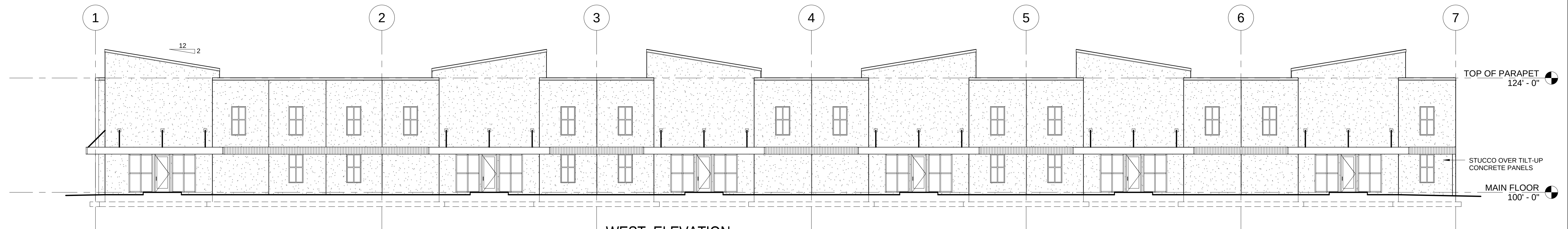
WEST ELEVATION
