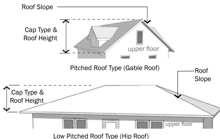
Figure 5.12 (2). Pitched Roof Type
